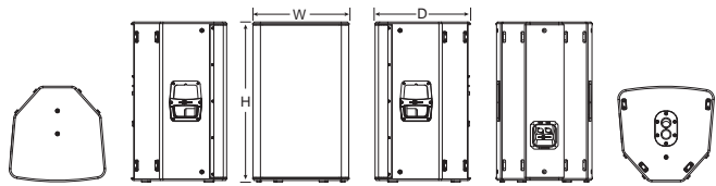
Dimension(WxHxD): 421x696x416mm
