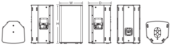
尺寸(WxHxD):355x599x349mm
