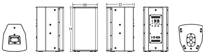
尺寸(WxHxD):245x447x320mm
