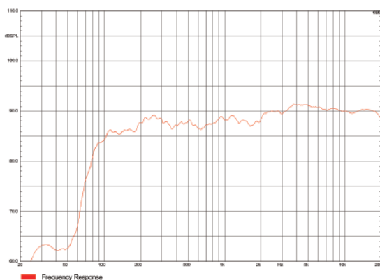
⊙ Artist T4 Frequency Response Curve
