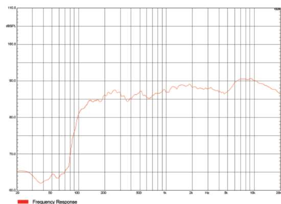
⊙ Artist T3 Frequency Response Curve
