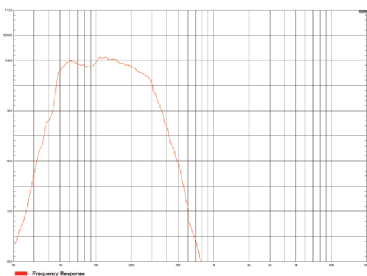
① Artist TW15频响曲线图
