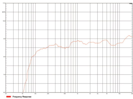
◎ Artist T4L频响曲线图
