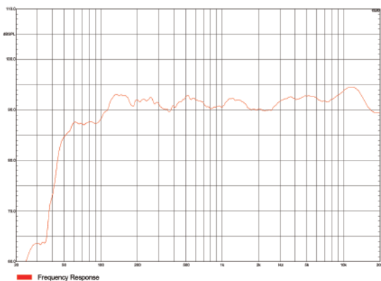
◎ Artist T8频响曲线图
