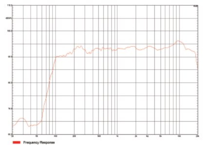
Artist T43频响曲线图
