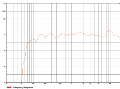
Artist T83频响曲线图
